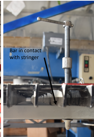
Figure 8b. C-clamp
