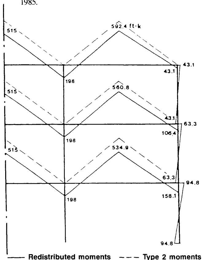
Fig. 12. Moment redistribution from modified type 2 procedure.
