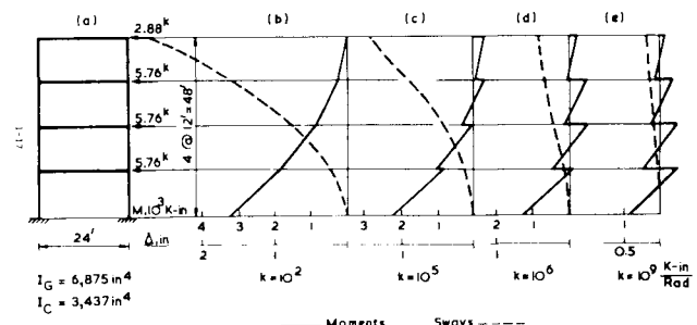
Fig. 3. Moments and sways of flexibly-connected steel frame.
