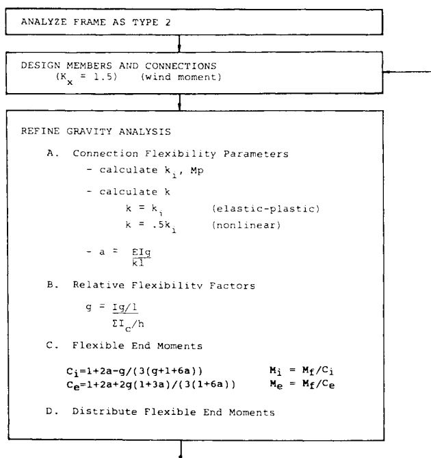
Fig. 11. Modified type 2 design steps.
