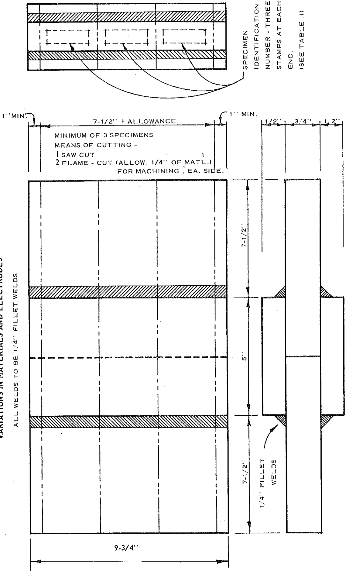
SPECIMEN BLANK - BEFORE MACHINING
