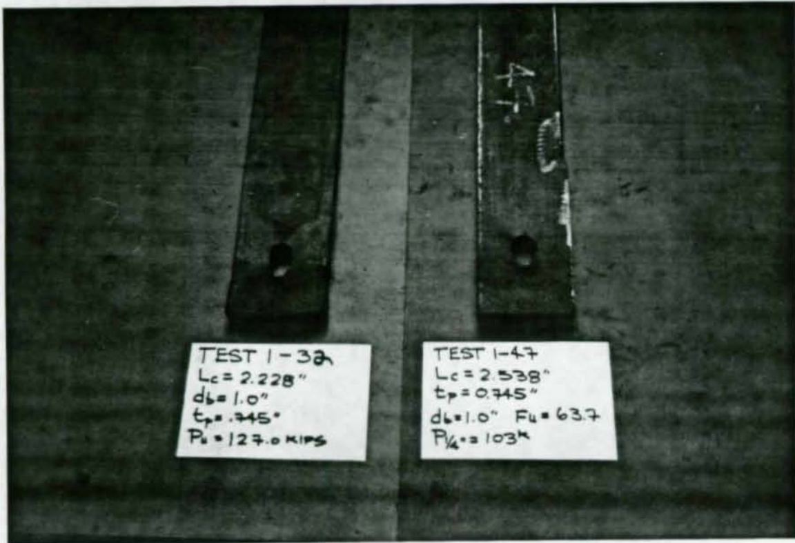
Figure 17. Two Failures for 1 in. Diameter Single-Bolt Specimens with Large End Distances. The specimen on the left was loaded through a large deformation, while the one on the right was stopped at 1/4 in. deformation. The maximum load for the specimen on the left is twenty-three percent higher than for the specimen on the right. There was a bolt failure during the test on the left; therefore, the result is not plotted.
