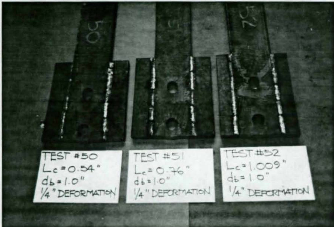
Figure 18. Comparison of 1/4 in. Deformations on Two-Bolt Specimens with 1 in. Diameter Bolts. The failure load for the specimen in the middle is 151 kips. This is less than the additive results from the specimens in Figures 16 and 17 (60.2 kips + 103 kips = 163.2 kips). The clear end distances for the specimens in Figures 16 and 17 are approximately equal to the clear end distance and clear spacing for the specimen in this figure.
