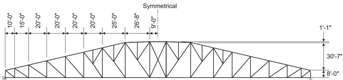
Figure 6 – Sample long span roof
