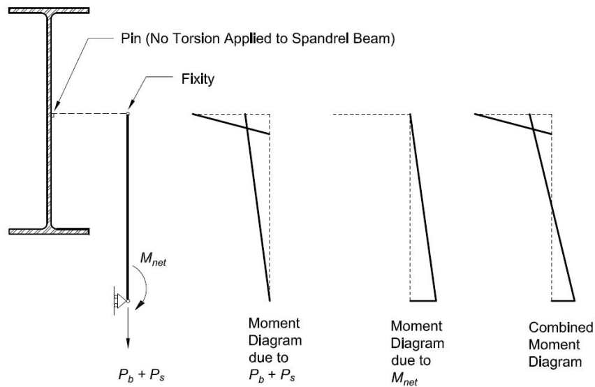
Fig. 7-28. Hanger assembly moment diagram with pin at spandrel beam web.
