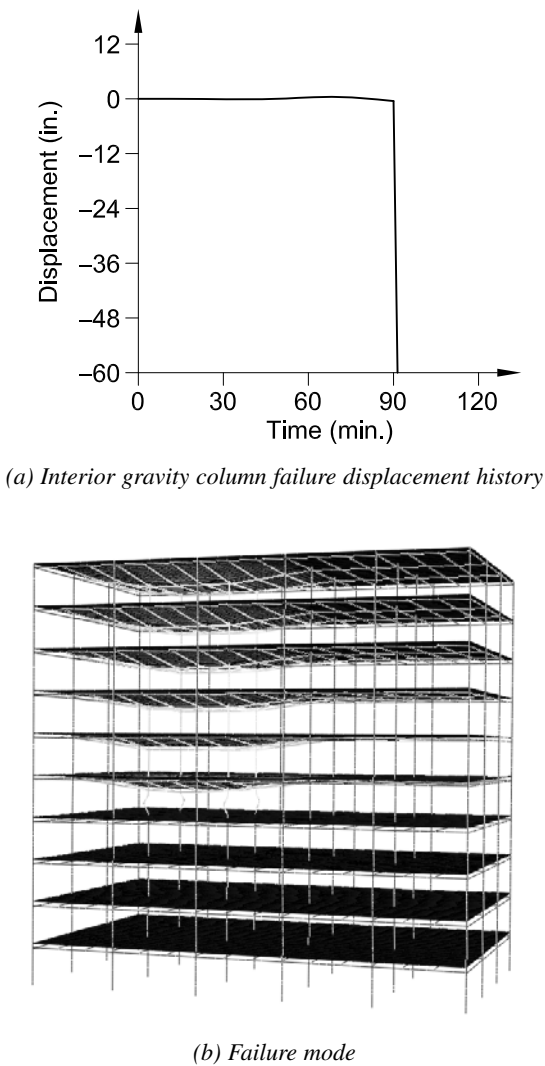
Fig. C-A-4.2. Advanced analysis of 3D building for design fire.
