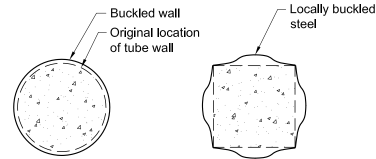
Fig. C-II.2. Cross-sectional buckling mode with concrete infill.
