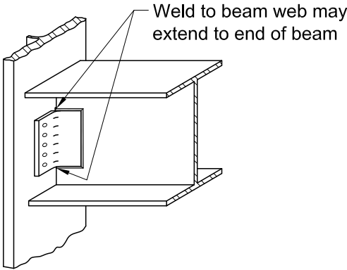
Fig. C-J2.6. Fillet weld details on framing angles.
