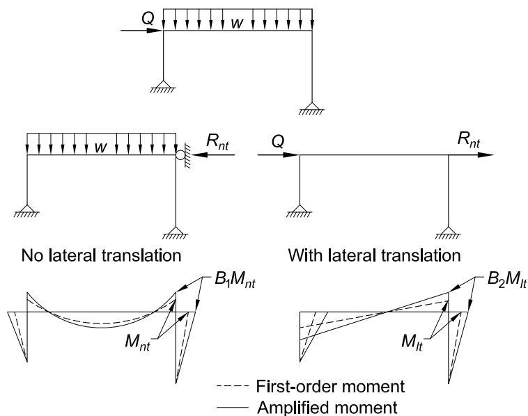
Fig. C-A-8.1. Moment amplification.
