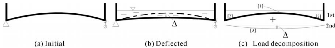
Figure 22 – Rain load on roof truss with camber
