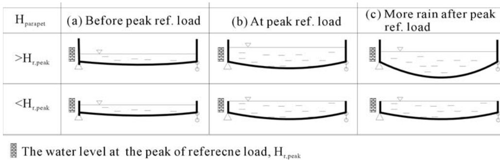
Figure 13 – Deflected shape of case 3
