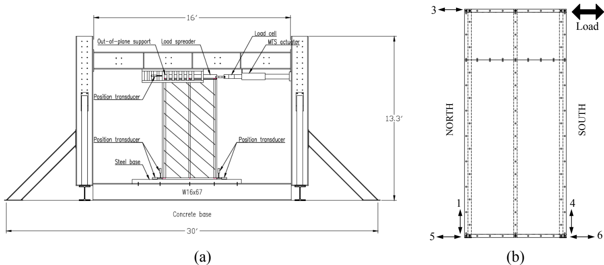
Figure 1: (a) Schematic of testing rig with specimen (b) Sensor plan where numbers correspond to position transducers measuring along the direction indicated by the arrows.
