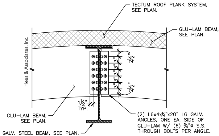
▲ A connection detail showing the intersection of glulam with wide-flange.
