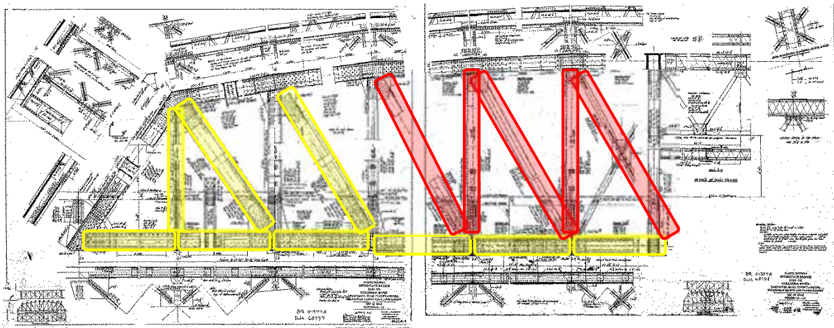
Fig. 3-7. Original design drawings for the identical spans (obtained from Oregon DOT).
