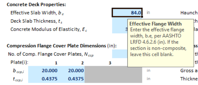
Fig. 4-3. Example showing yellow message windows that appear when clicking on input cells.
