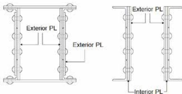
Fig. 2-1. Illustration showing examples of “interior” and “exterior” web plates.
