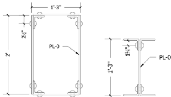
Fig. 3-8. Cross sections for members L0-L1 (left; showing stay plates) and U1-L1 (right).
