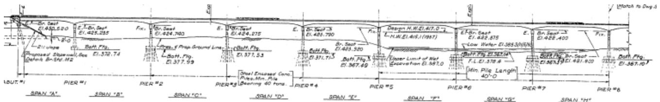
Fig. 4-7. Original design drawings for the 1958 built-up riveted two-girder bridge.
