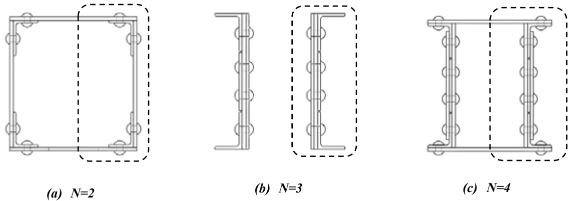
Fig. 2-4. Examples of plate counts, N , for bending factor, \Xi_B .
