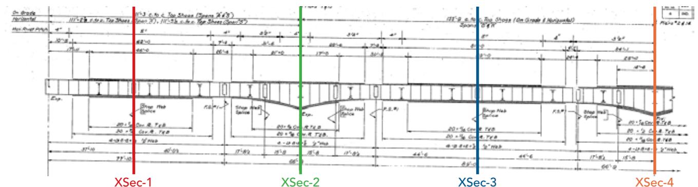
Fig. 4-8. Elevation view of the built-up riveted girders.
