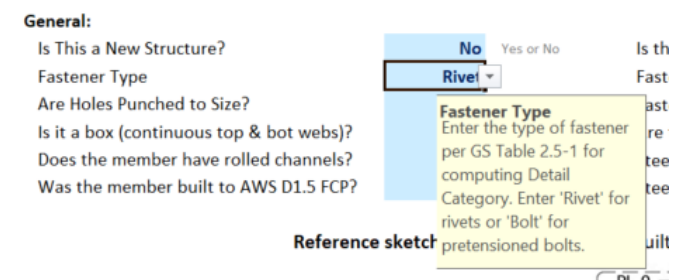
Fig. 3-3. Example showing yellow message windows that appear when clicking on input cells
