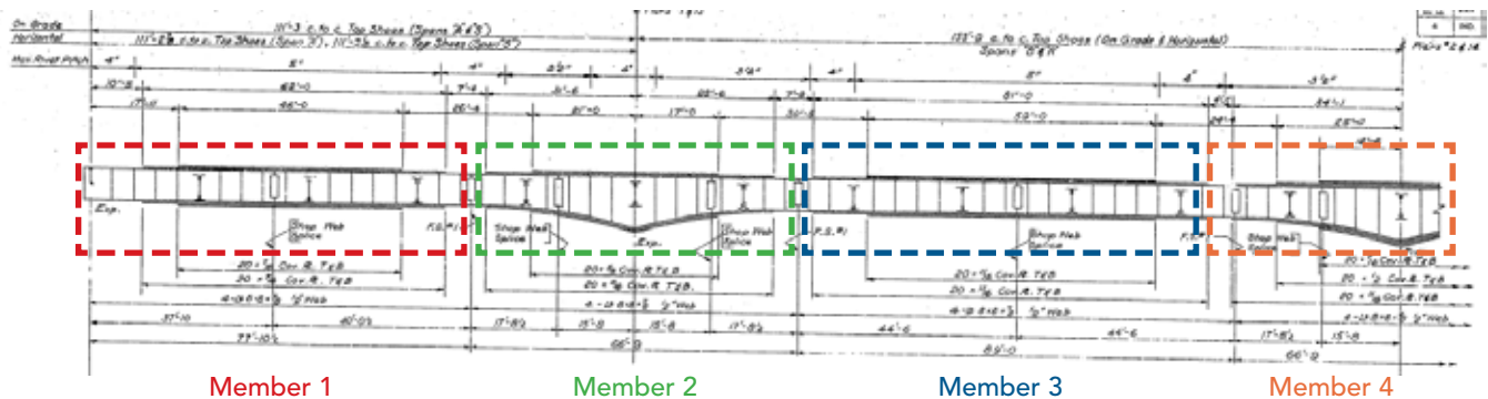
Fig. 4-19. Example of how to subdivide continuous girder for evaluation and inspection of IRMs.
