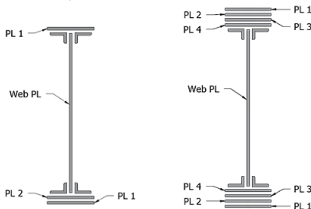
Fig. 4-5. IRM Flexural Evaluator spreadsheet reference sketches illustrating proper cover plate labels.
