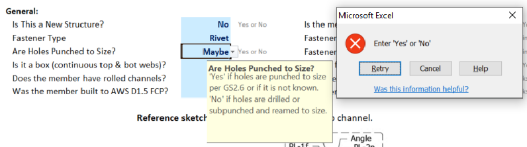
Fig. 3-4. Example warning message for incorrect value entered.
