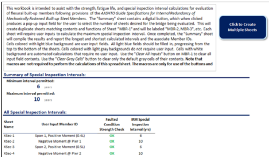
Fig. 4-1. Screenshot showing the summary sheet within the IRM Flexural Evaluator.
